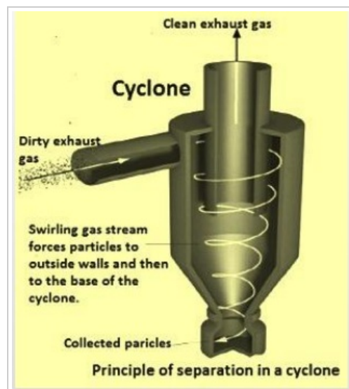
Fig. 7 — A cyclone separator: the swirling gas stream forces coarse particles to the outer wall and down into a collection hopper.
