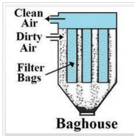
Fig. 8 — A baghouse: dirty air is blown through fabric filter bags; particulates are trapped while clean air exits at the top.
