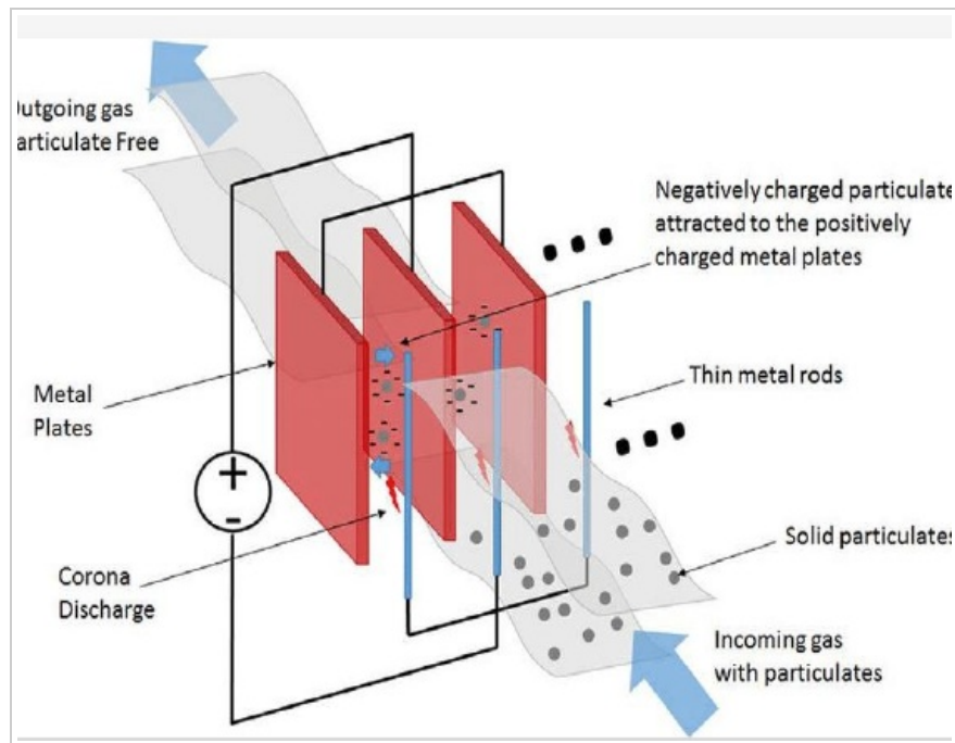
Fig. 4 — Working of an electrostatic precipitator: charged metal plates attract negatively charged particulates via corona discharge, leaving clean outgoing gas.
