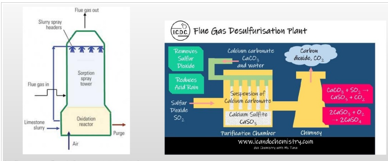
Fig. 5 — Flue gas desulfurization: (left) wet scrubbing sorption spray tower; (right) limestone-based FGD plant removing \text{SO}_2 and reducing acid rain.
