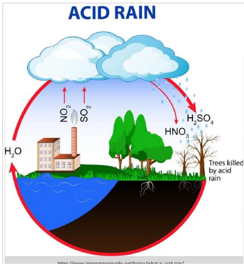
Fig. 3 — Formation cycle of acid rain: \text{SO}_2 and \text{NO}_2 react with atmospheric moisture to form \text{H}_2\text{SO}_4/\text{HNO}_3 , which fall as acid rain and kill vegetation.
